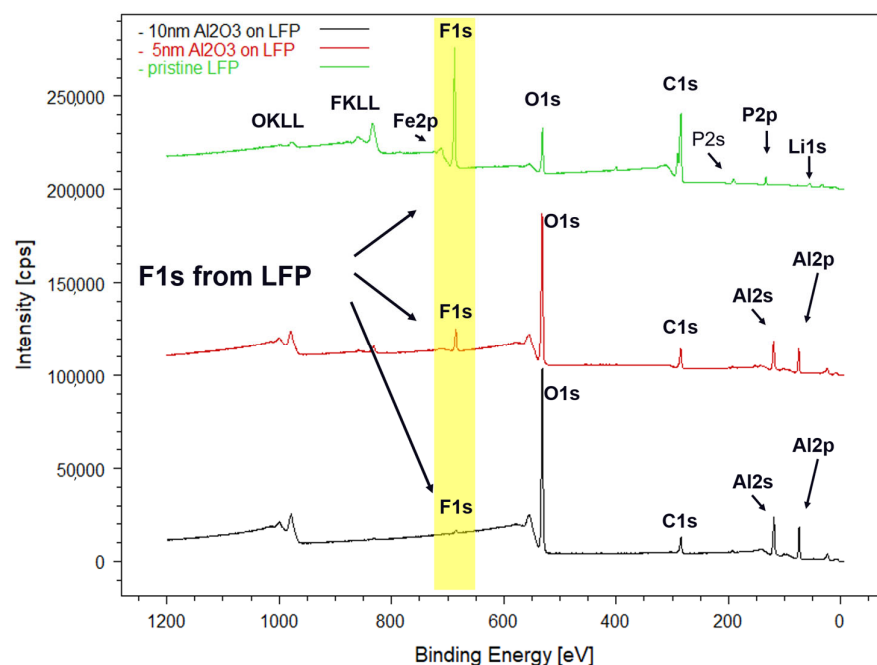
Figure 1. XPS survey spectra of the pristine LFP (green curve), LFP coated with 5 nm Al 2 O 3 (red curve), and LFP coated with 10 nm Al 2 O 3 (black curve). The main core levels are labeled.
