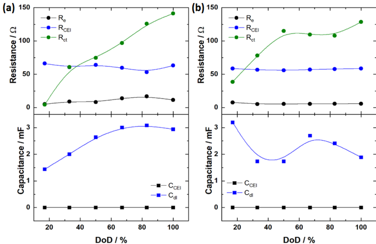
Figure 7. Resistance and capacitance obtained from fitting the EIS spectra at different states of lithiation for the pristine LFP electrode (a) and 5 nm Al_2O_3 -coated LFP electrode (b).
