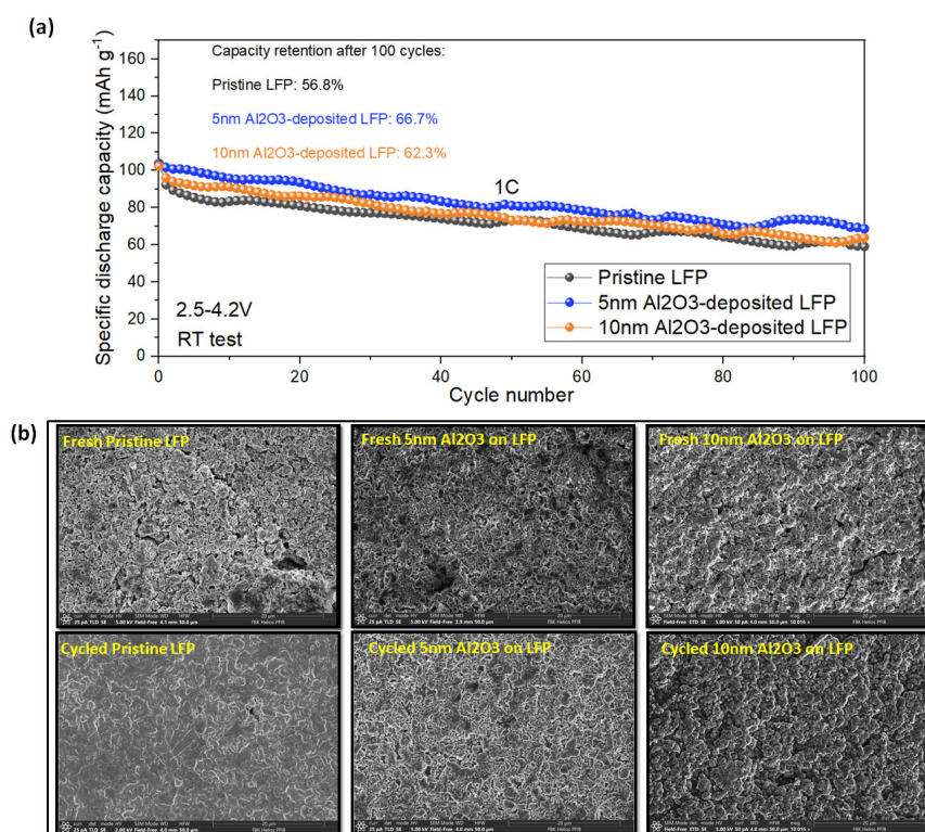
Figure 3. (a) Cycling performance of Li/LFP cells with and without \text{Al}_2\text{O}_3 deposition, in the range of 2.5–4.2 V at 1C ( 1\text{C} = 170 \text{ mA g}_{\text{LFP}}^{-1} ) and RT. The test was performed after 10 cycles at 0.1C. (b) Top-view FE-SEM images of the electrodes in the fresh state and 100 cycles at 1C.
