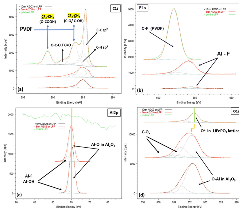
Figure 2. XPS core-level spectra of (a) C1s, (b) F1s, (c) Al2p, and (d) O1s, acquired on the pristine LFP (green curve), LFP coated with 5 nm \text{Al}_2\text{O}_3 (red curve), and LFP coated with 10 nm \text{Al}_2\text{O}_3 (black curve). The main core-level components are labeled.
