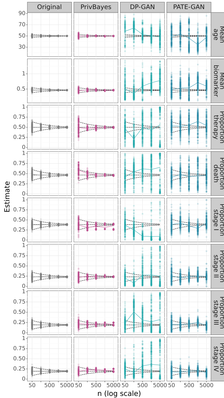
Figure E1: Simulation study results for all mean and proportion estimators. Each dot is an estimate per Monte Carlo run (200 dots in total per value of n ). The population parameter is represented by the horizontal dashed line. The dashed funnel indicates the behaviour of an unbiased and \sqrt{n} -consistent estimator based on observed data.
