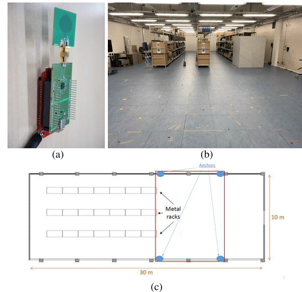
FIGURE 2. The measurements were performed in the open space area of the IIoT-lab at Ghent University which simulates an industrial environment. (a) The UWB hardware platform for the data collection [6], (b) the IIoT-lab environment, and (c) the ground plan of the environment.
