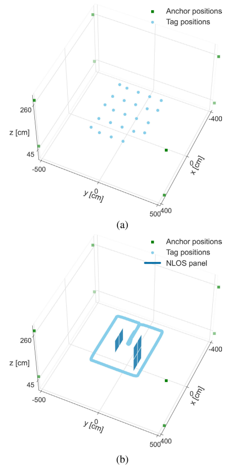
FIGURE 4. Both static (a) and dynamic (b) trajectories are collected in the iiot-lab. The dynamic scenario covers realistic sharp corners and areas with high numbers of NLOS links are created with the absorbing panels.
