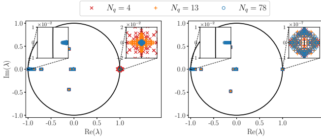
Fig. 2. Spectrum of the companion matrices for the TD-PMCHWT (left) and the TD-EFIE (right) on a sphere. The shift \delta of eigenvalues near 1 + 0j of the TD-PMCHWT decreases when increasing the number of quadrature points N_q , whereas that of the TD-EFIE is independent of quadrature rules (see Table I for further details). The eigenvalues near -1 + 0j are not problematic as they reside strictly inside the unit circle [16].
