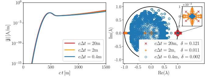
Fig. 5. MOT solutions (left) and spectrum of the companion matrices (right) for the TD-PMCHWT on a sphere. The shift \delta of eigenvalues near 1 + 0j increases linearly with \Delta t , but the growth of solution over time is independent.
