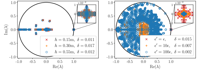
Fig. 6. Spectrum of the companion matrices for the TD-PMCHWT on a sphere. (Left) The surface is triangulated with different mesh sizes h . (Right) Different interior permittivities \epsilon' are used. The shift \delta of eigenvalues around 1 + 0j is not significantly affected by h , while it decreases when increasing the material contrast.
